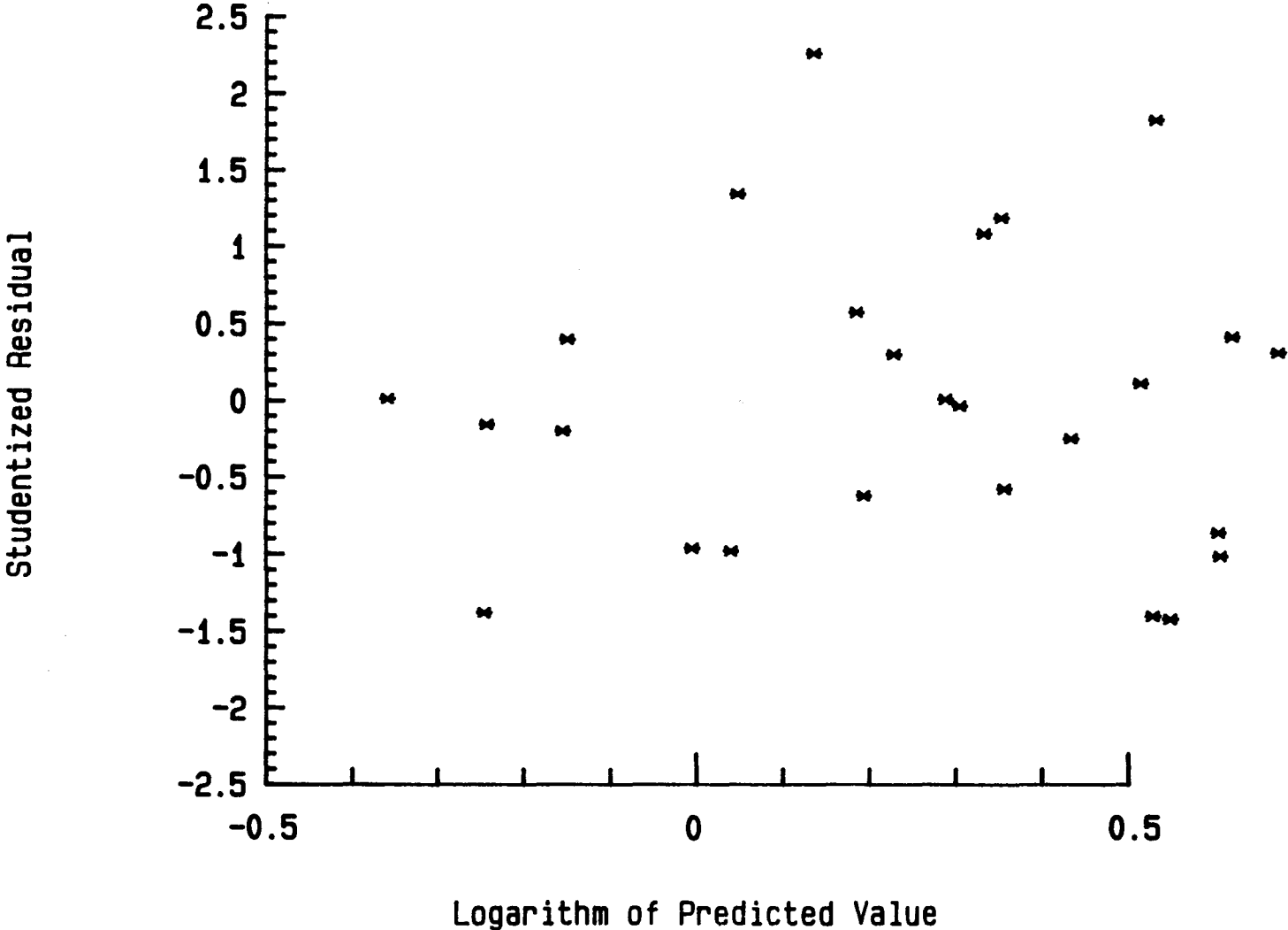
Skeena River Data Untransformed Heteroscedastic Model
