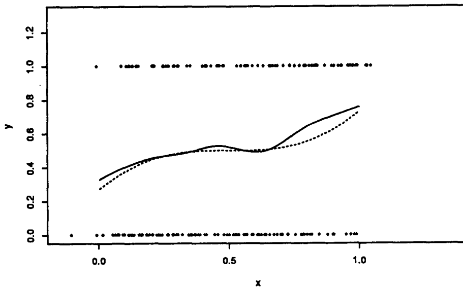
Figure 11. Scatterplot of the responses and the covariates contaminated with double exponential errors ( r = 0.90 ). The solid curve is the estimate (2.1) and (2.9) with h_n = 0.1 . The dotted curve is the underlying regression function \text{logit}(Y|X^\circ = x) = 8(x - 0.5)^3 .
