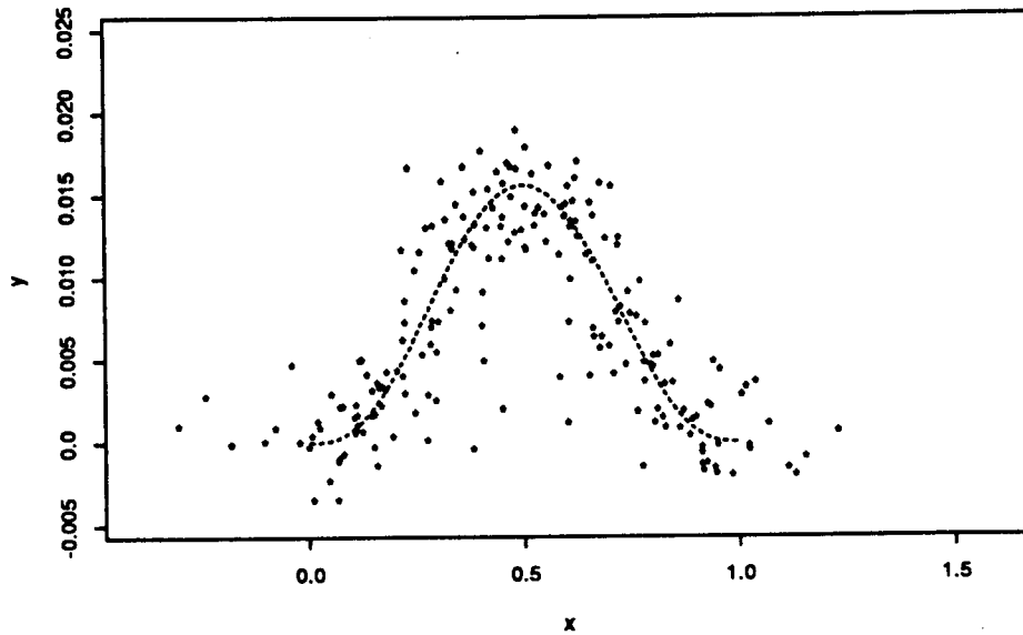
Figure 7. Scatterplot of the responses and the covariates contaminated with double exponential errors ( r = 0.80 ).
