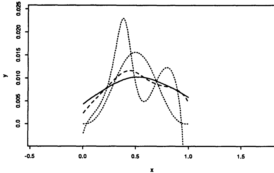
Figure 6. Deconvoluted kernel estimates: normal errors with r = 0.70 . The solid, dash and the dotted curves are the estimates with c = 1.0 , c = 0.80 and c = 0.60 , respectively. The true regression function is also plotted for comparison.
