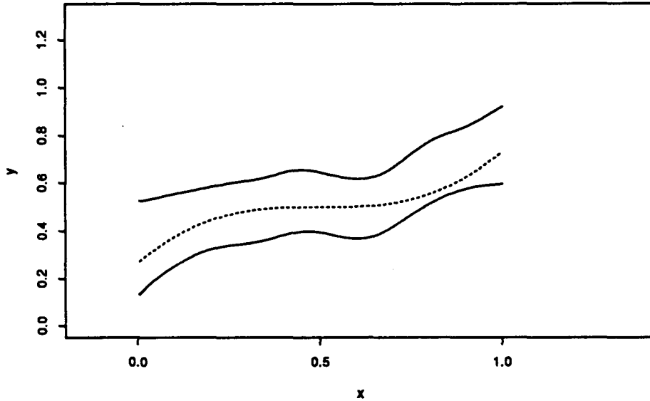
Figure 15. 95% pointwise confidence intervals for \text{logit}(Y|X^\circ = x) = 8(x - 0.5)^3 . Based on the binary response data in Figure 11.
