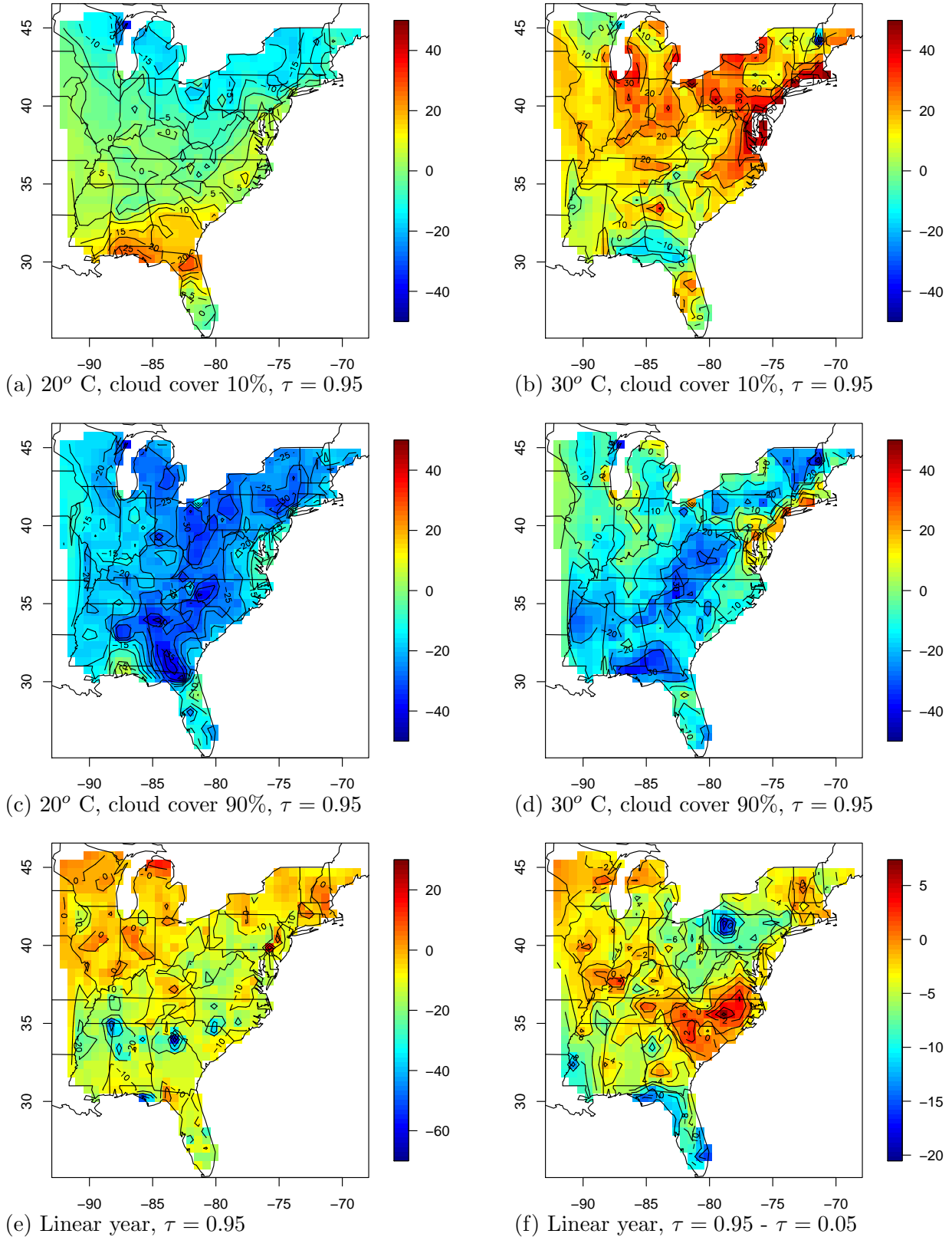
Figure 4: Summary of the posterior mean of \beta_j(\tau, s) . Panels (a)-(d) plot linear combinations of \beta_j(\tau, s) as discussed in (21). Panel (f) plots the posterior mean of \beta_j(0.95, s) - \beta_j(0.05, s) . The units are parts per billion in all plots.
