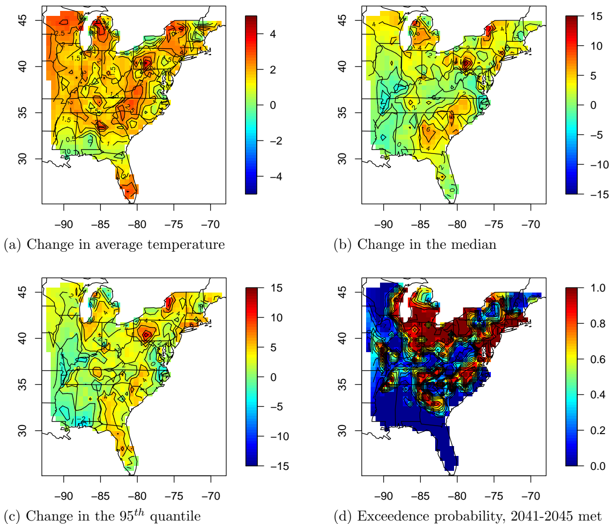
Figure 7: Panel (a) plots the change in average temperature between the calibrated 2041-2045 data and the observed 1997-2005 data. Panels (b) and (c) plot estimates of the change in yearly median and 95 th quantile the future and current climate scenarios (standard errors are less than 3ppb for all sites and quantiles). Panel (d) gives the probability that the three-year (2041-2043) average of the fourth-highest daily maximum 8-hour average ozone concentrations exceeds 75 ppb for future climate scenario.
