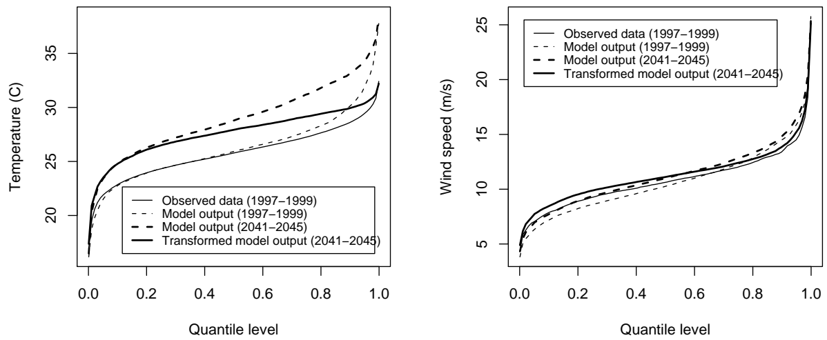
Figure 5: Calibration plots for meteorological data in Georgia.
