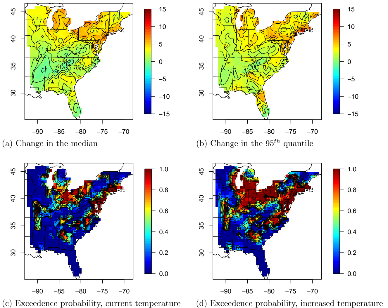
Figure 6: Panels (a) and (b) plot estimates of the change (ppb) in yearly median and 95 th quantile due to shifting each daily average temperature by 2°C (standard errors are less than 3ppb for all sites and quantiles). Panels (c) and (d) give the probabilities that the three-year (2003-2005) average of the fourth-highest daily maximum 8-hour average ozone concentrations exceeds 75 ppb for current temperature and the 2°C increase in temperature, respectively.
